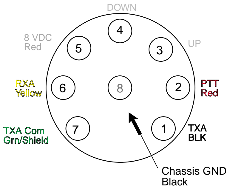
Kenwood 8-Pin MIC Plug (Female PLUG) viewed from Solder end
